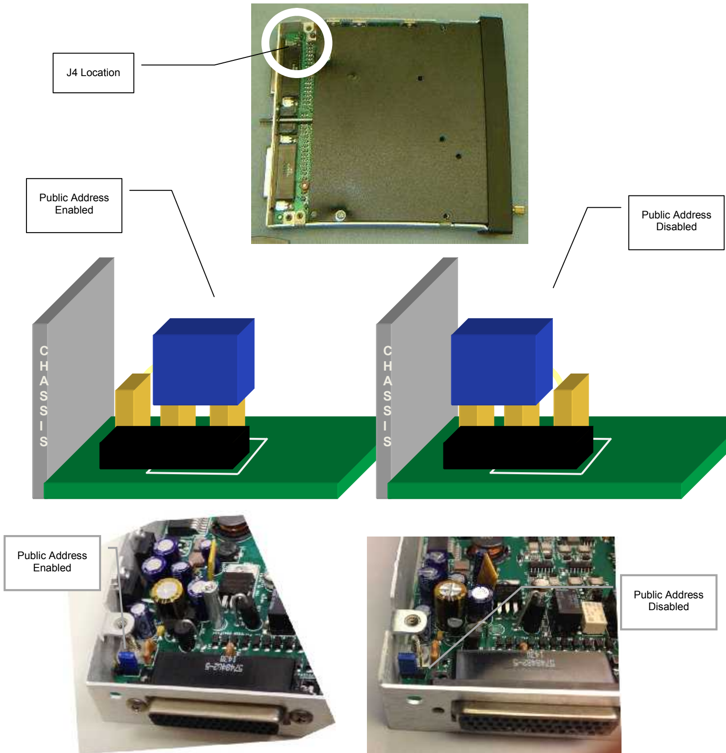
Figure 2-3 Jumper Locations
