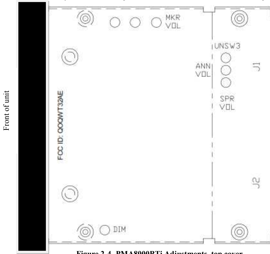
Figure 2-4- PMA8000BTi Adjustments, top cover
