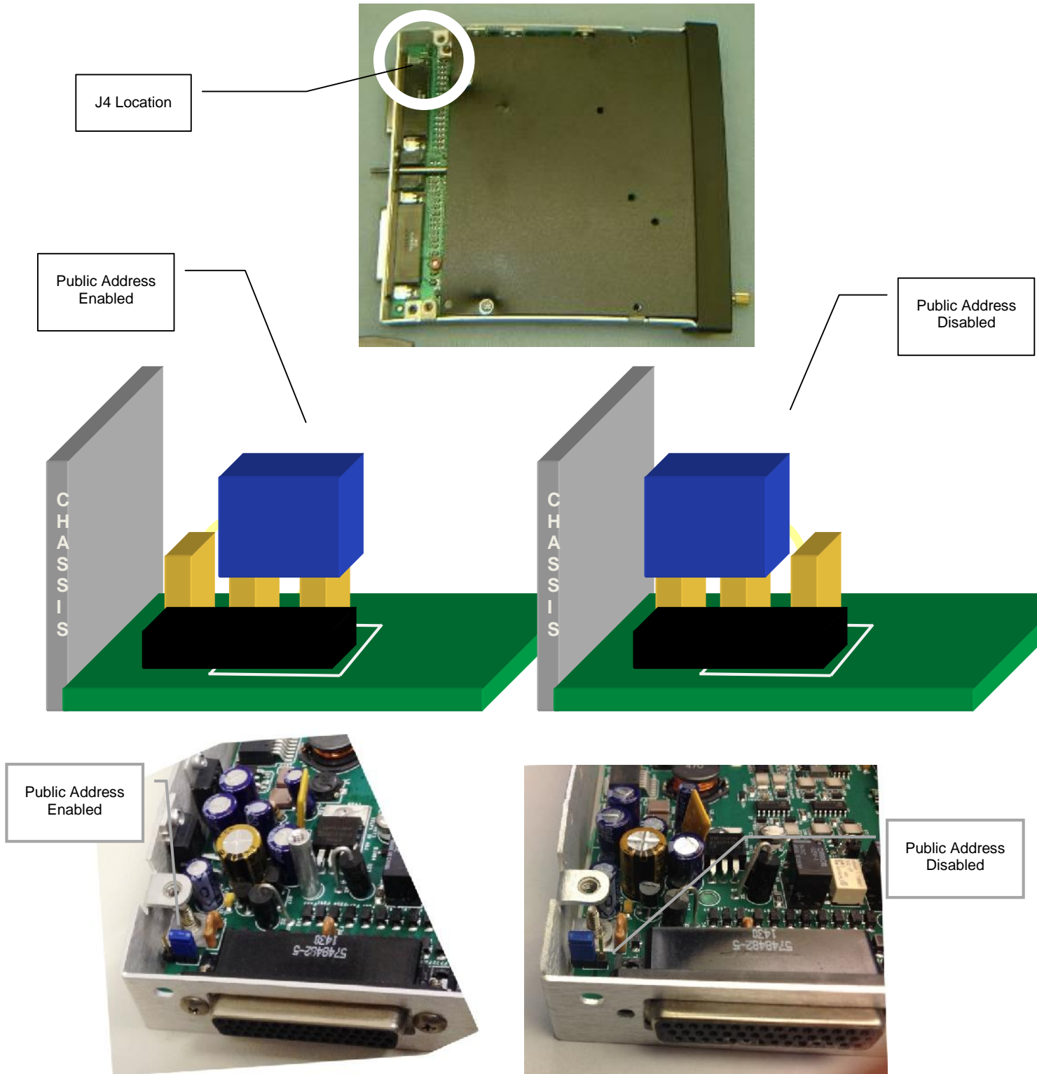
Figure 2-3 Jumper Locations
