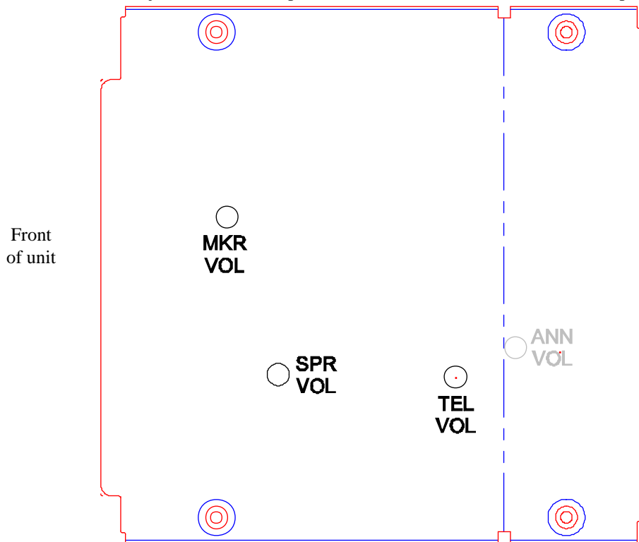
Figure 2-4- PMA8000BT Adjustments, top cover
